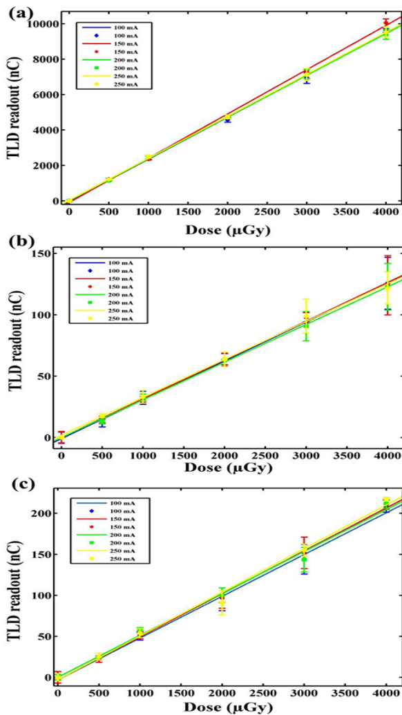
Figure 2: The dose-response curves of GR-200 (a), TLD-700H (b) and TLD-100 (c) for various values of current tube in 0.5-4 mGy dose range at 1 day after irradiation. The standard deviations in a number of points are low; hence, the error bars are often not seen clearly.
