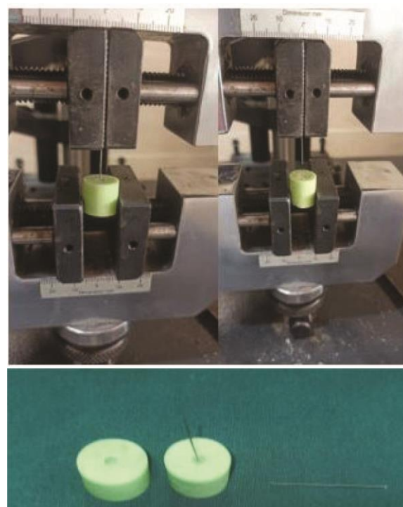
Figure 3: The instruction of pull-out test
