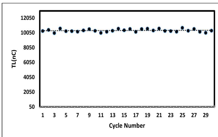
Figure 4: Reproducibility test of Thermoluminescent Dosimeter (TLD) reader of model TR5500 for 30 annealing-expose-readout cycles
