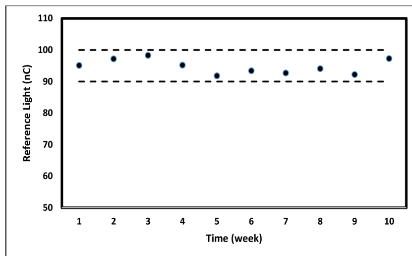
Figure 3: Stability of Photo Multiplier (PM) tubes Thermoluminescent Dosimeter (TLD) reader of model TR5500
