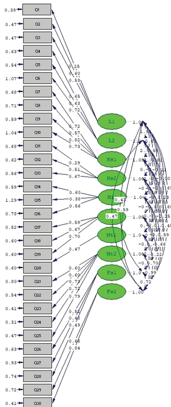
Figure 1: Confirmatory factor analysis for evaluating the questionnaires.
